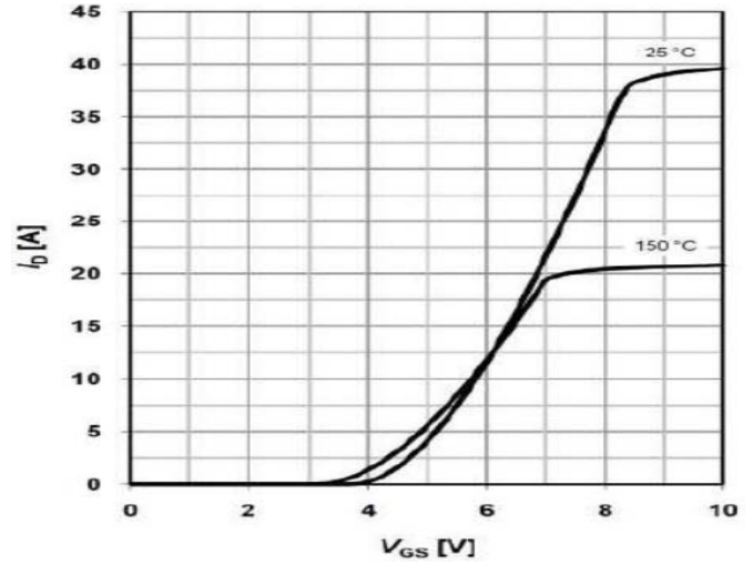
Transfer Characteristic
