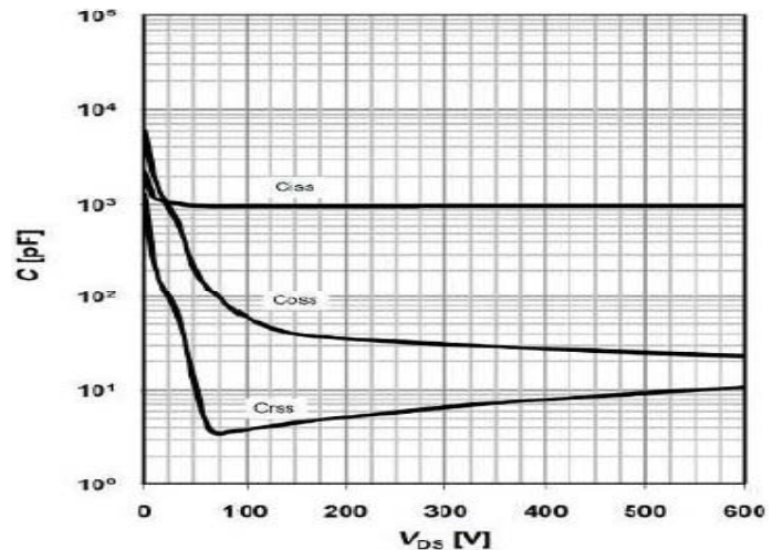
Capacitance
