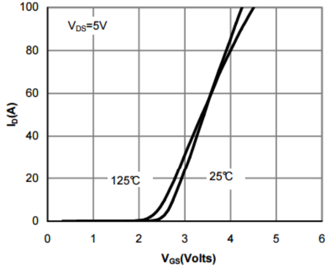
Transfer Characteristic
