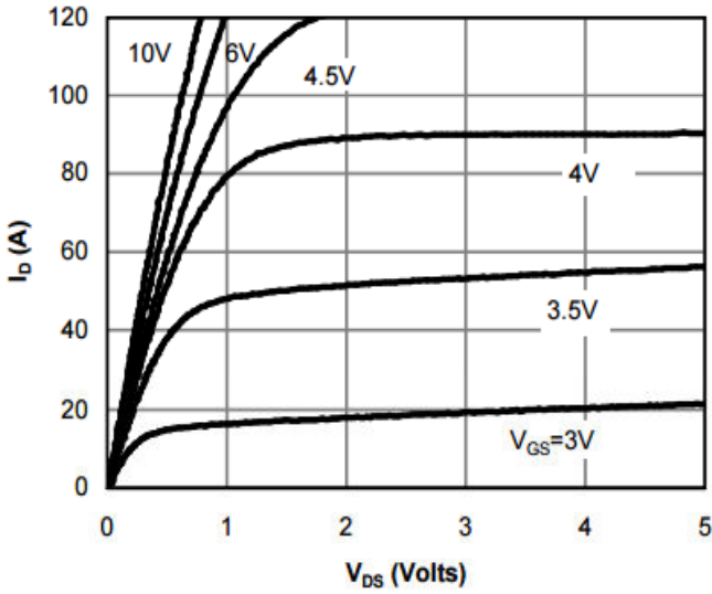
Output Characteristic
