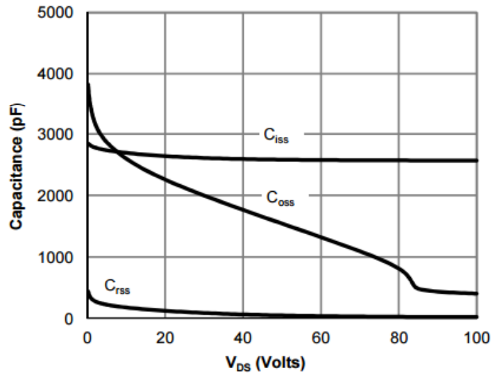
Capacitance
